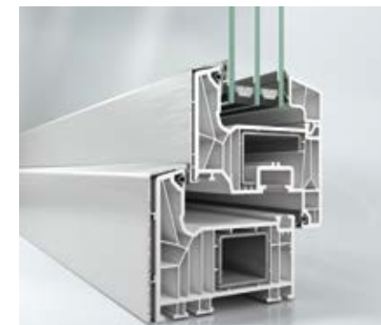
TopAlu Classic
